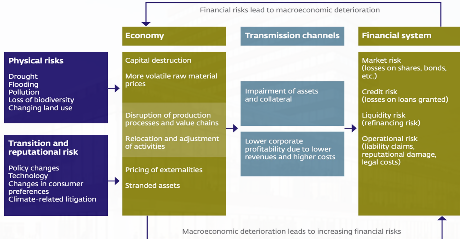
Figure 2 From sustainability risks to financial risks
